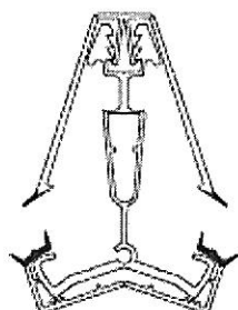
Georgian Bar height 91mm
