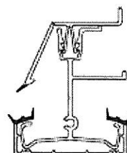
Starter Bar height 65mm
