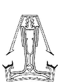
Transom/Victorian Bar height 78mm
