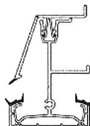
Starter Bar height 78mm
